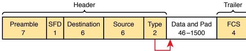
Figure 5-2 IEEE 802.3 Ethernet Frame (One Variation)
