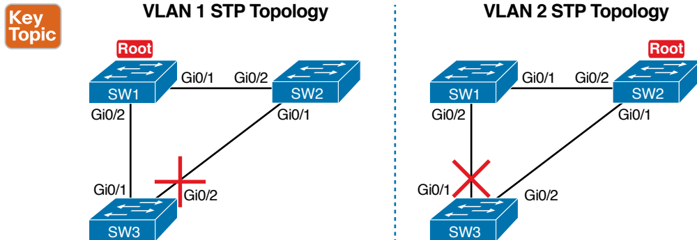
Figure O-2 Load Balancing with PVST+
