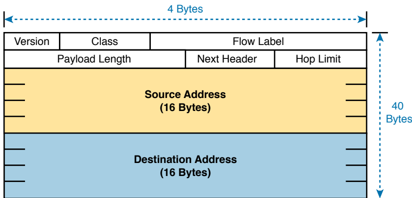
Figure 22-3 IPv6 Header
