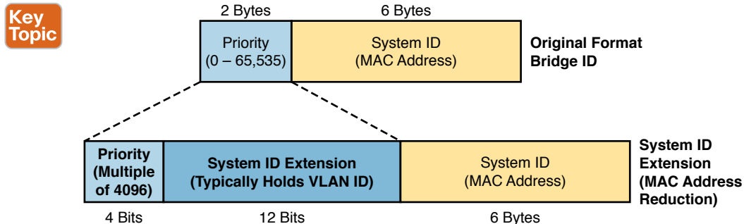
Figure O-3 STP System ID Extension
